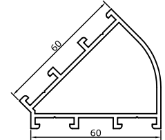
4150 135° Dönüş Profili 135° Corner Profile 1,180 kg/m
