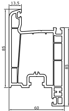
607 Dar Kapı Kanat Profili Tight Door Sash Profile 1,520 kg/m
