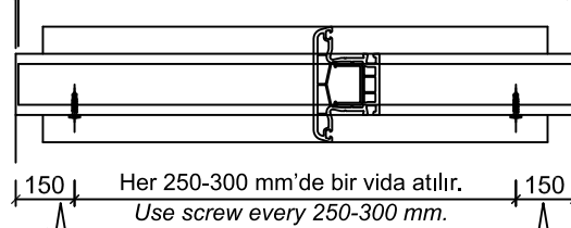
Destek Sacı Kesim Boyu = (B-D) Reinforcement Cutting Length (B-D)
