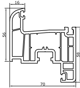
7003 Kanat Profili Sash Profile 1,440 kg/m
