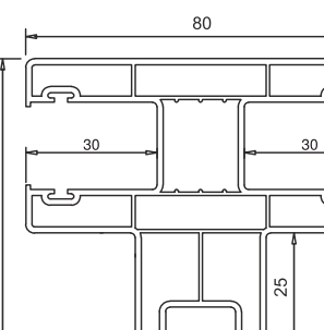
MNB.250.3T.9014 Ön - Üst - Arka Profil Front - Top - Back Profile MNB.250.1T.9016 Alt Profil Bottom Profile
