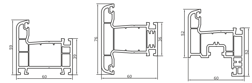
401 Kasa Profil Frame Profile 0.909 kg/m 402 Orta Kayıt Mullion Profile 1.028 kg/m 403 Kanat Profil Sash Profile 1.090 kg/m 471 Pervazlı Kasa Profil Wide Frame Profile 1.000 kg/m
