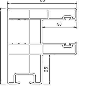
MNB.197.3T.9016 Üç Kapama Profil Front - Top - Back Profile MNB.197.1T.9016 Alt Profil Bottom Profile
