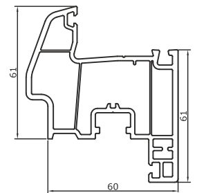
4504 İnce Bağ Profil Connection Profile 0.390 kg/m (Al) / 0.380 kg/m (PVC)
