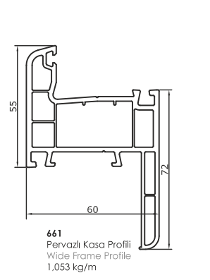
631 Kasa Profil Frame Profile 0.990 kg/m 632 Orta Kayıt Mullion Profile 1.090 kg/m 633 Kanat Profil Sash Profile 1.270 kg/m 661 Pervazlı Kasa Profil Wide Frame Profile 1.053 kg/m
